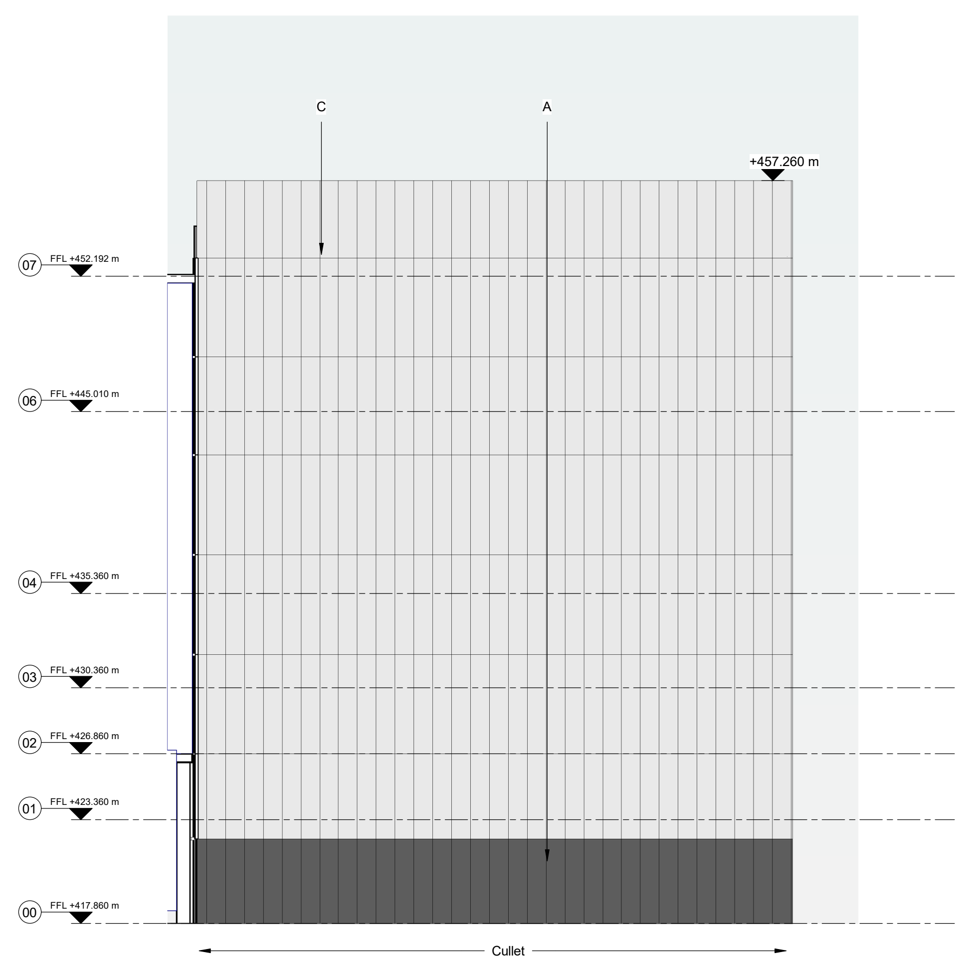
2 Elevation Cullet - North 1:200
