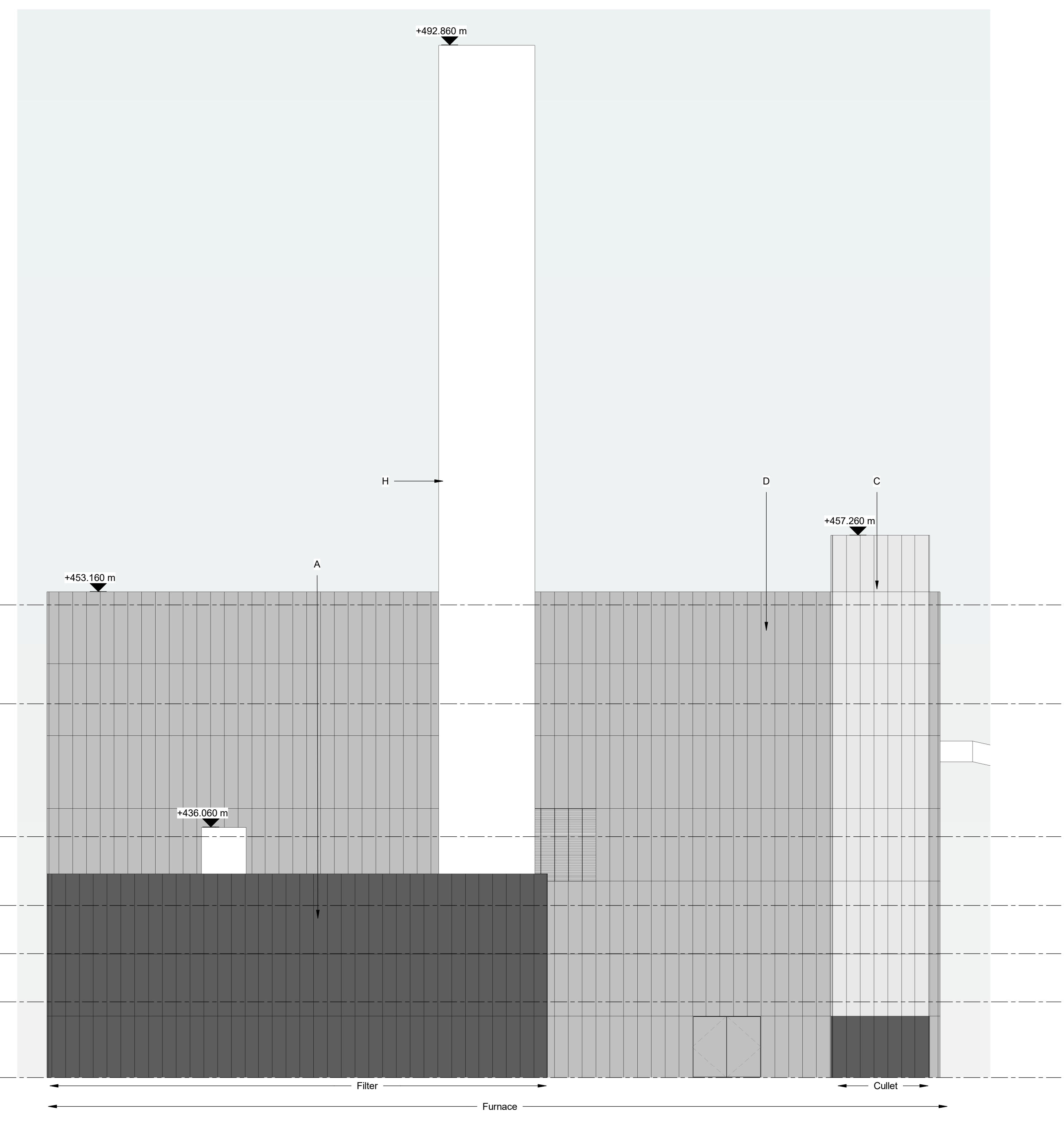
4 Elevation Filter & Cullet - West 1:200
