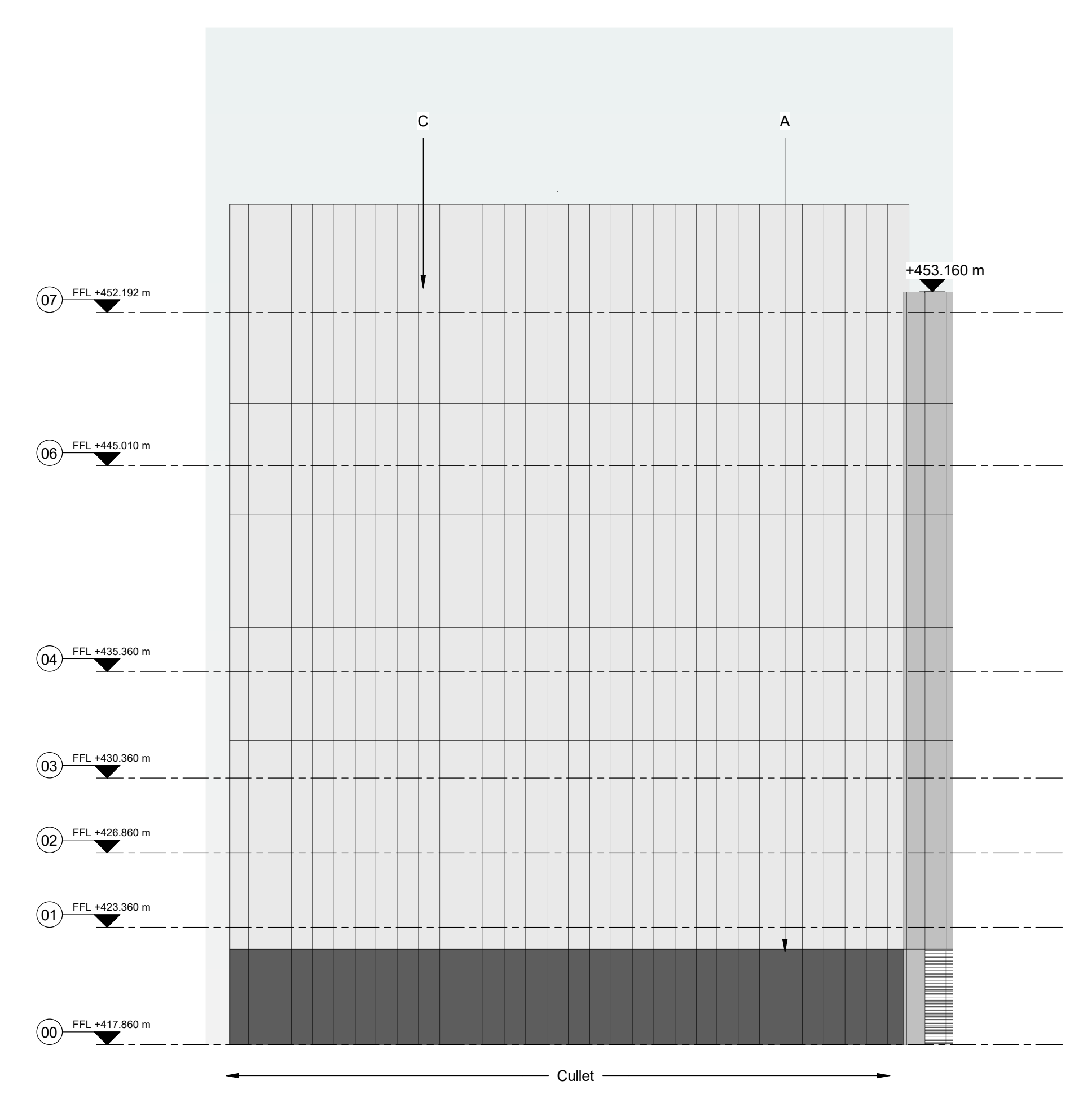
3 Elevation Cullet - South 1:200
