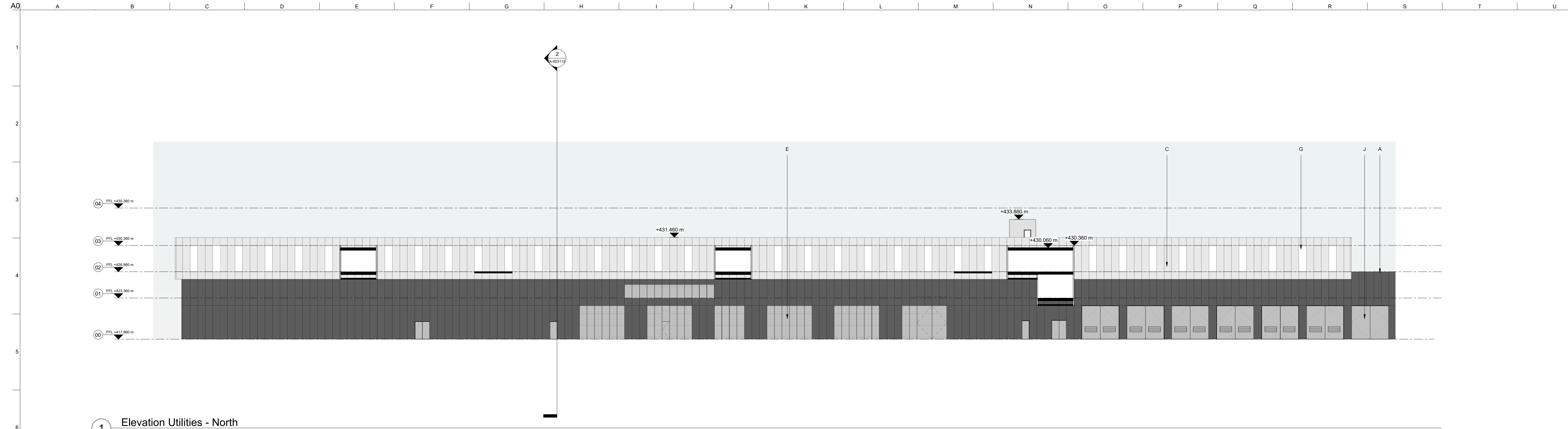
1 Elevation Utilities - North 1 : 200
