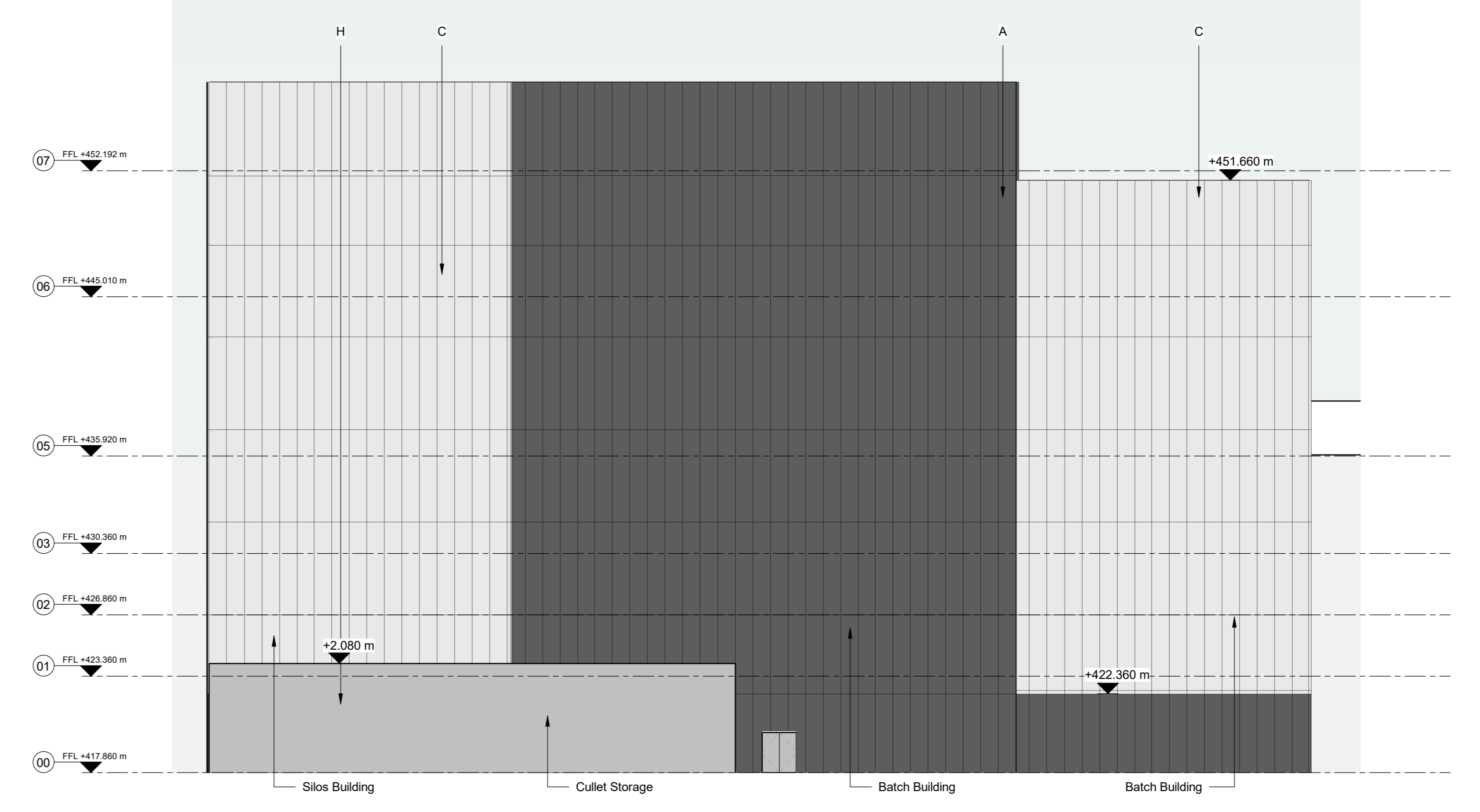
2 Elevation Batch - South 1 : 200
