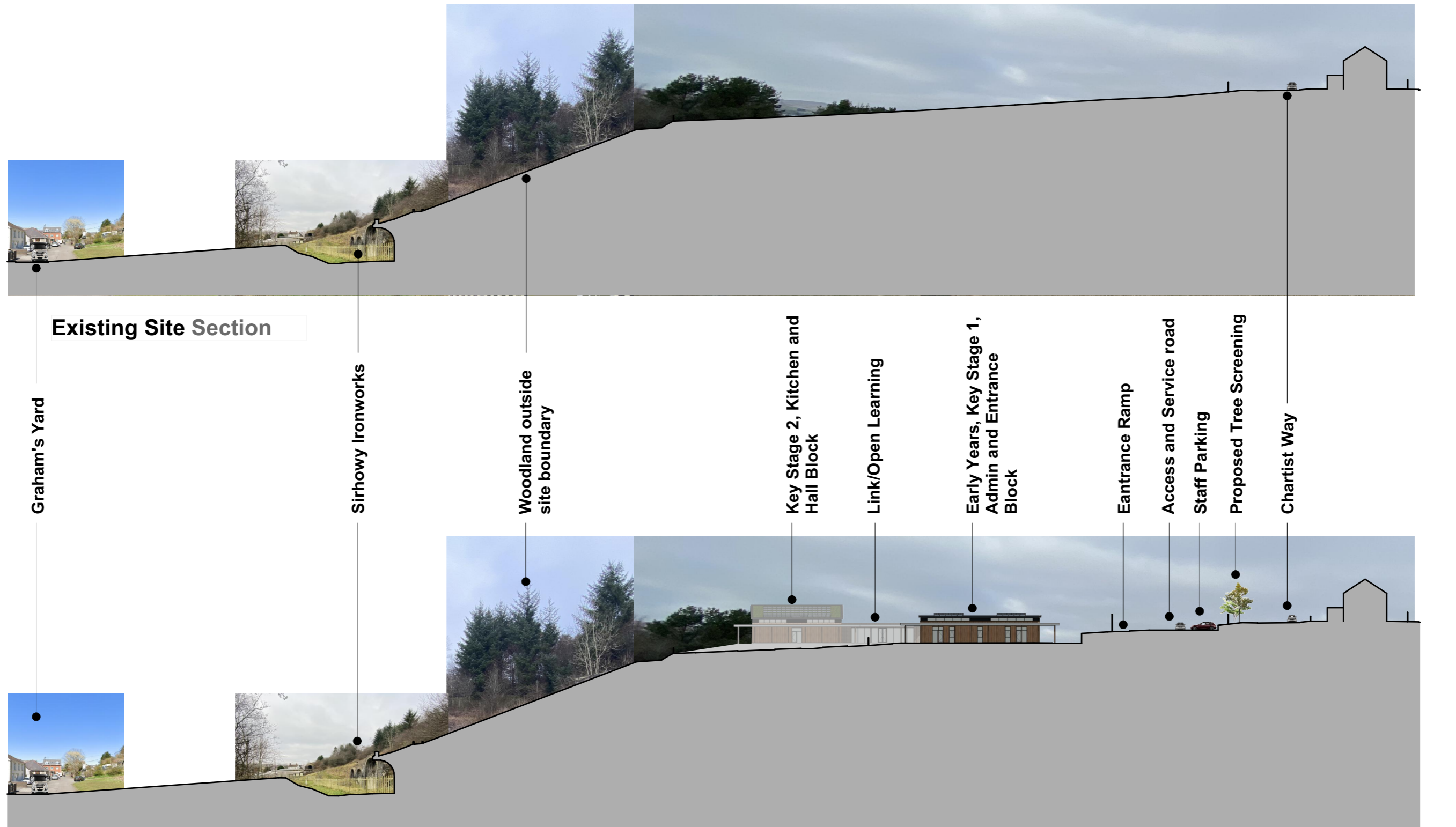
Proposed Site Section
