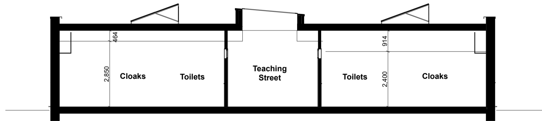
Building Section 3
