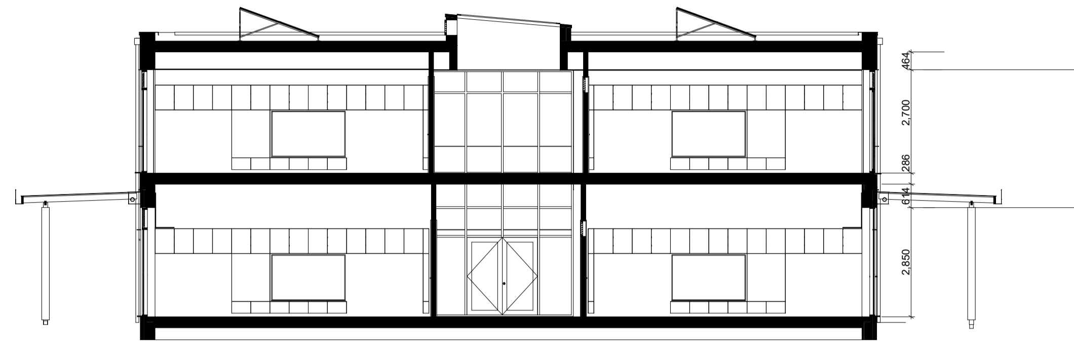
Building Section 1
