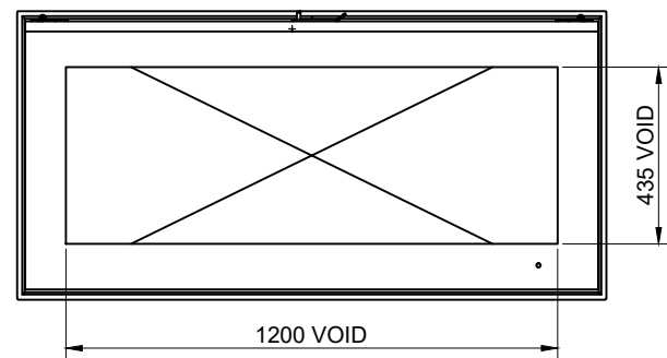
GRP ENCLOSURE DETAILS
