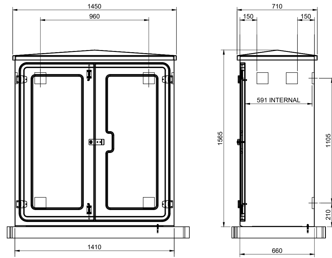
GRP ENCLOSURE DETAILS
